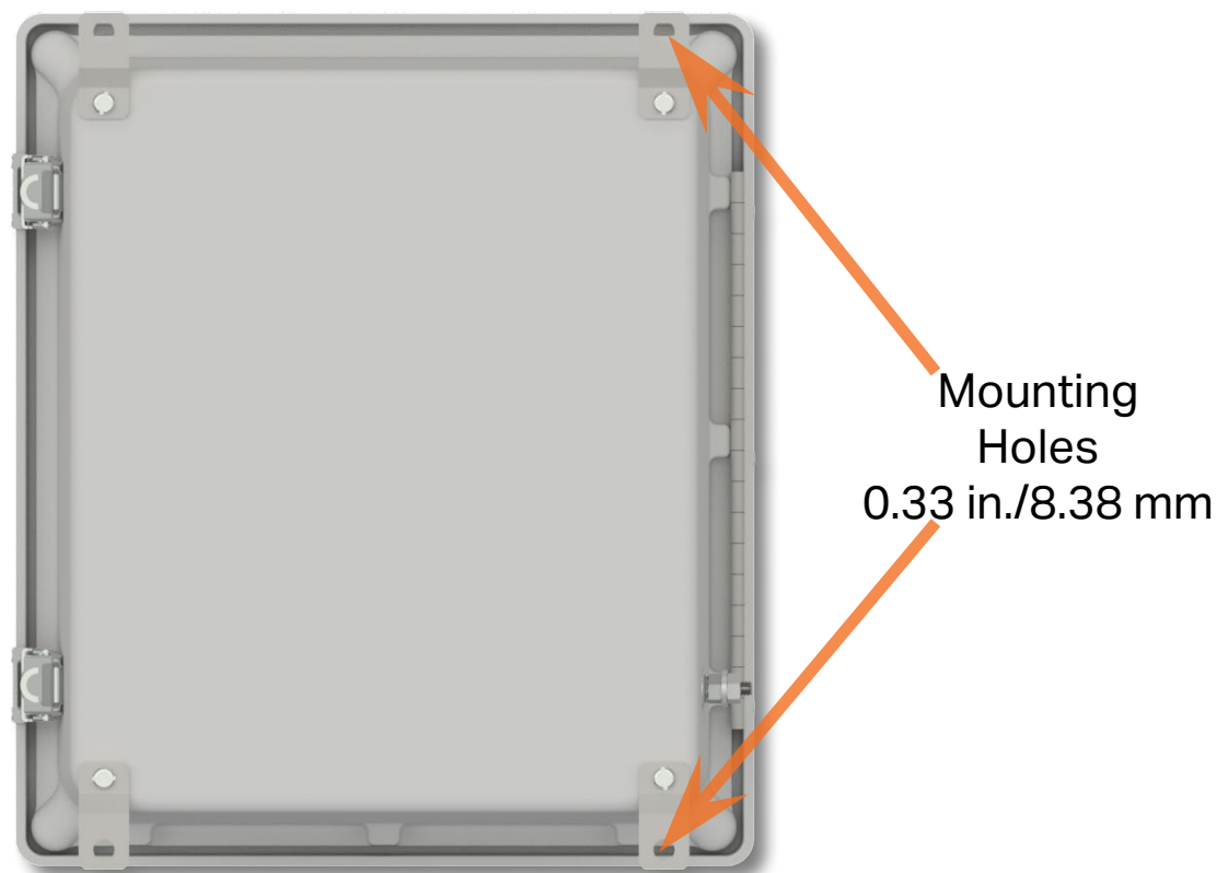
Figure 3. SCE100 Series Rear View
