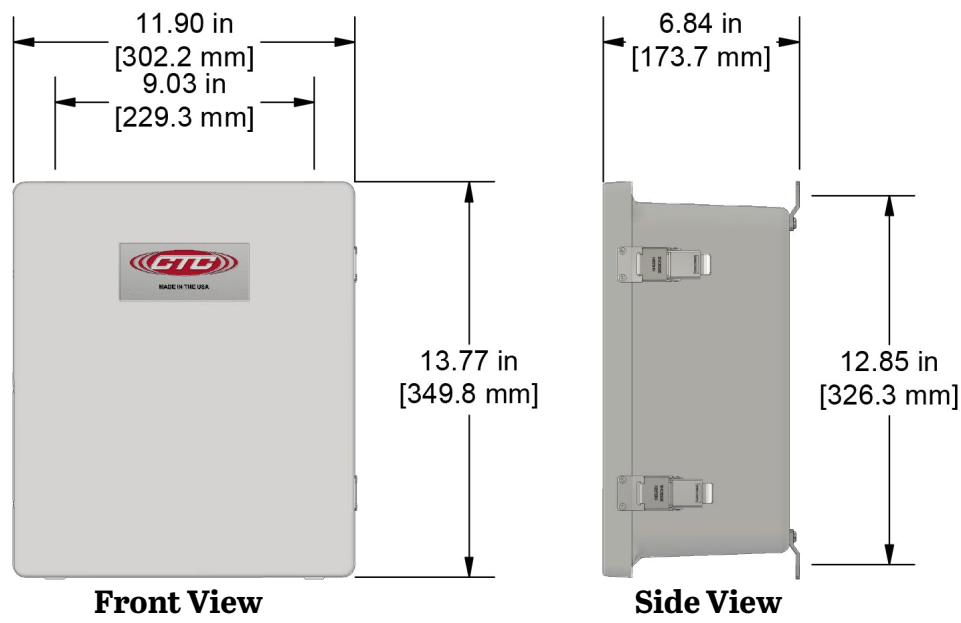
Figure 1. Dimensions
