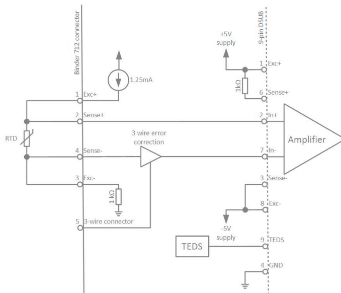
Basic circuit design of DSI-RTD
