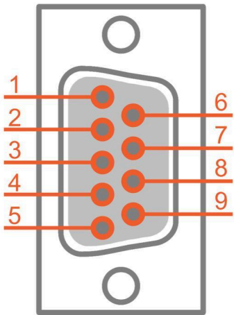
9 pin DSUB female
