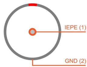
ACC connector: pin-out (BNC)
