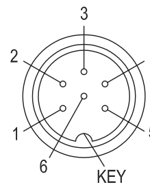
Front View of Connector
