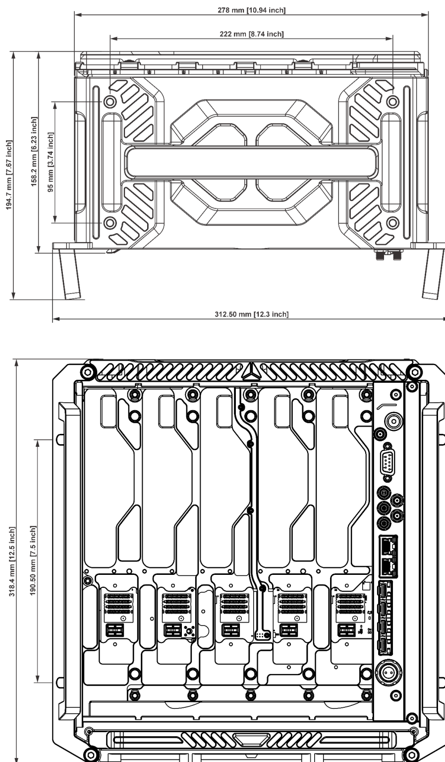
XR5 mechanical drawing
