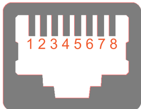
EtherCAT IN connector: pin-out (RJ45)
